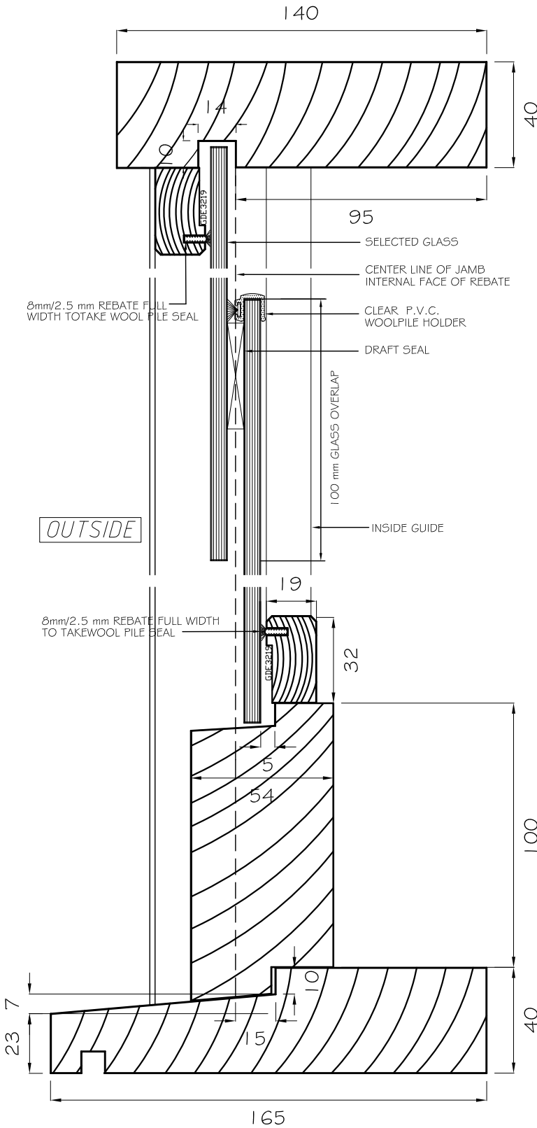
SILL DETAIL
