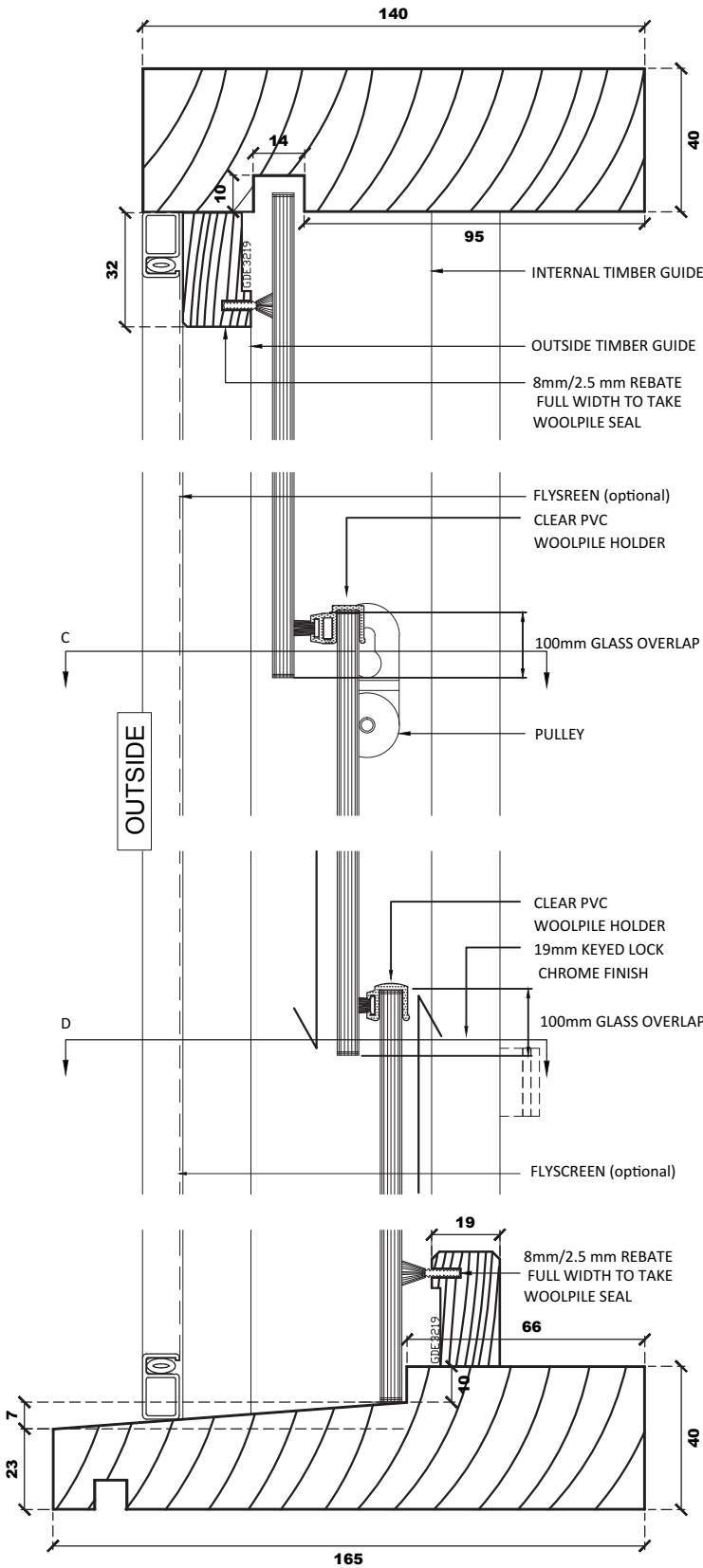
DETAIL (A) Head Detail
