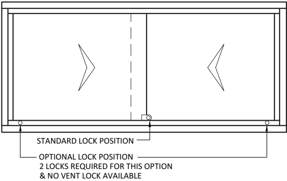
Typical Elevation (internal)
