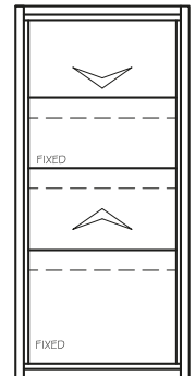
4 PANEL DOUBLE HUNG BOTTOM AND CENTRE FIXED 4PBCF
