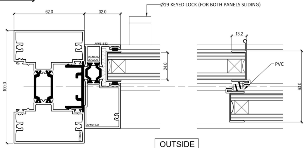
Interlock Detail
