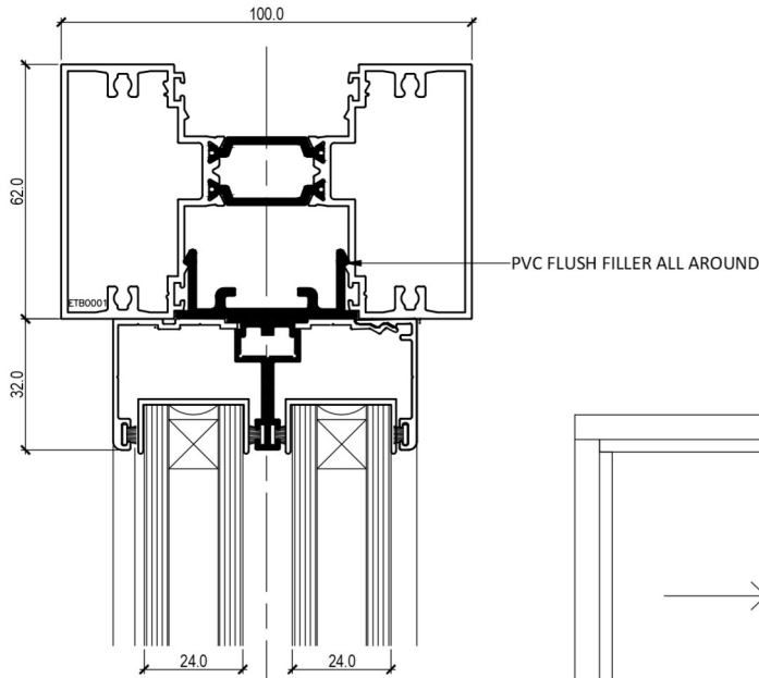
Head Detail
